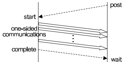
Figure 1. MPI-2 Communication with Active Synchronization
