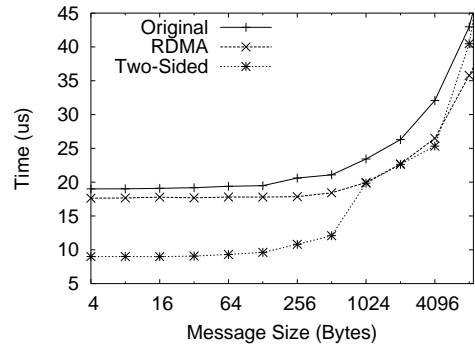
Figure 6. Bi-Directional Test
